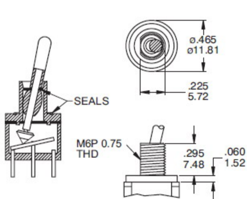
B9 SPLASH PROOF
