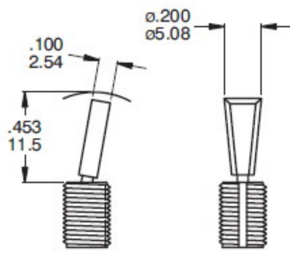
T6 FLATTED WITH ANTIROTATION
