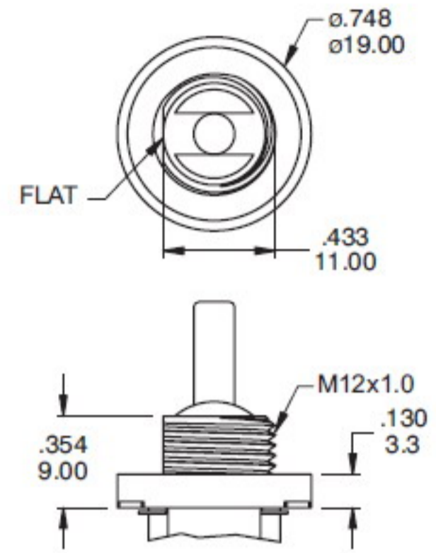
BA1 SPLASH PROOF
