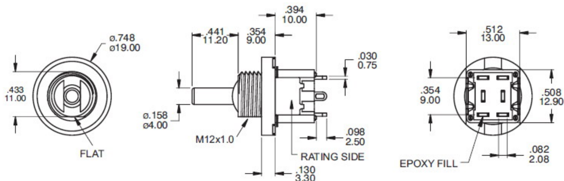
Part No. Shown : 1FD1T12BA1M1QES
