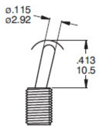
T6 FLATTED WITH ANTIROTATION
