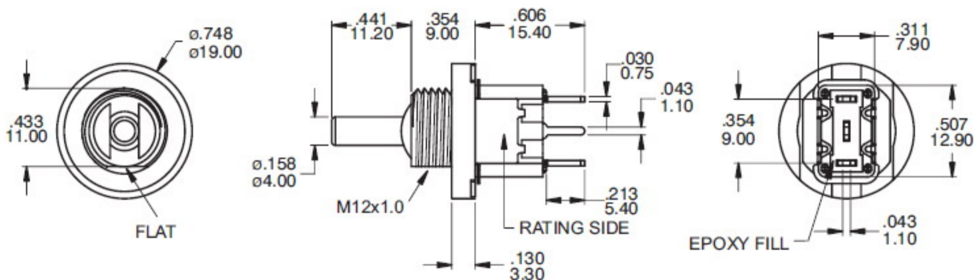
Part No. Shown : 1FS1T12BA1M2QES
