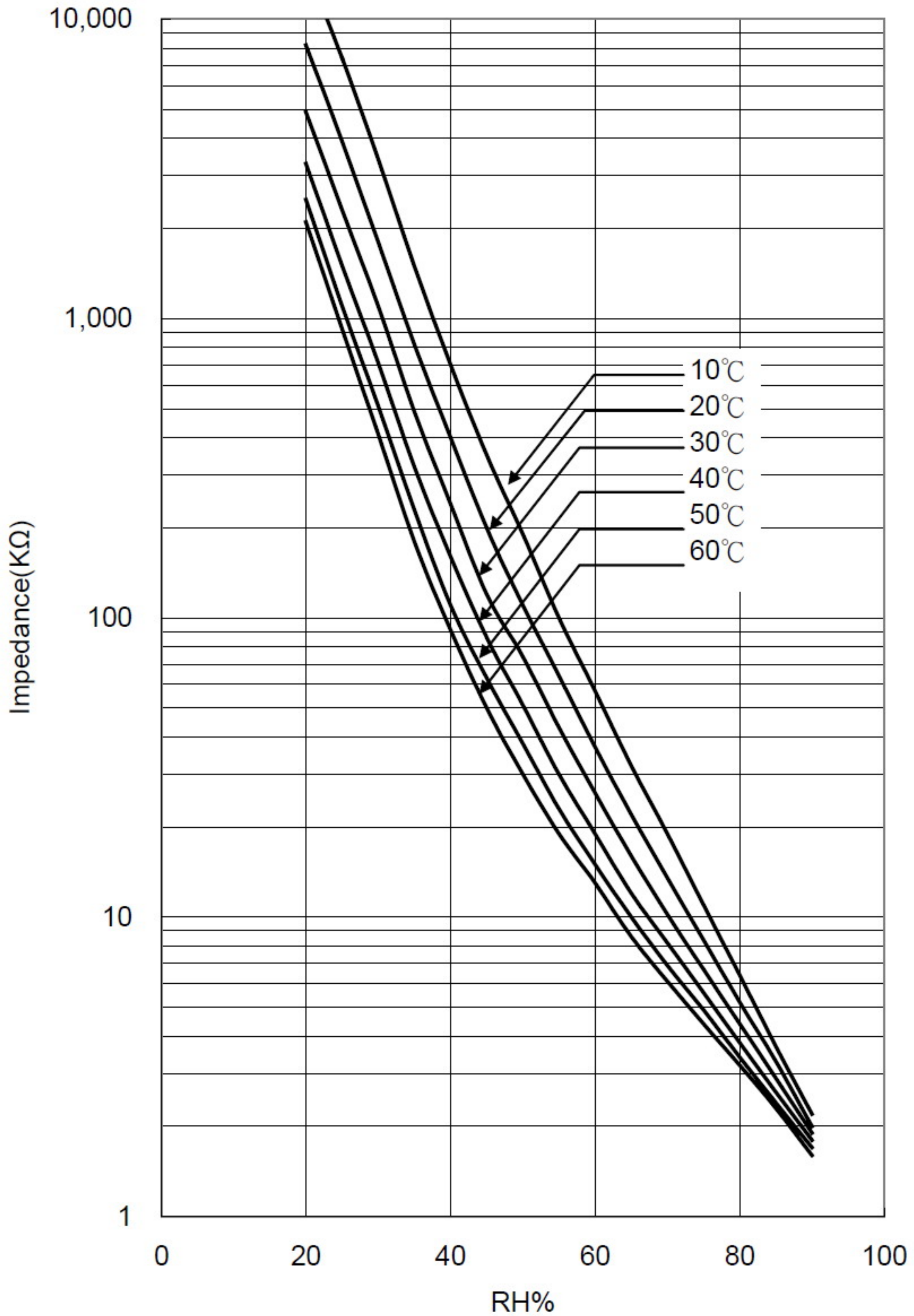
Impedance -- %RH VS. Temperature
