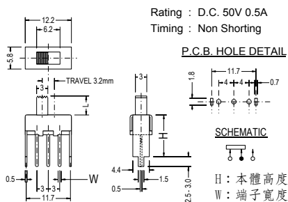
ON-ON(1P2T)
